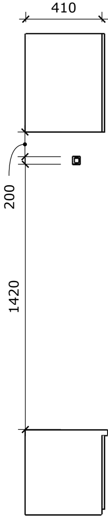
Bokorys
